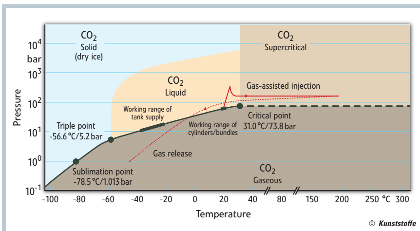
Fig. 2. The phase diagram for carbon dioxide shows the thermodynamics of the CO 2 gas-assisted injection technique where the gas is supplied from cylinders or cylinder bundles
