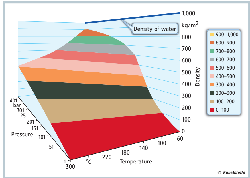
Fig. 1. The density of CO 2 as a function of pressure and temperature. CO 2 can be liquefied at room temperature by raising the pressure to 60 bar; as the pressure rises, its density approaches that of water (source: Maximator)
